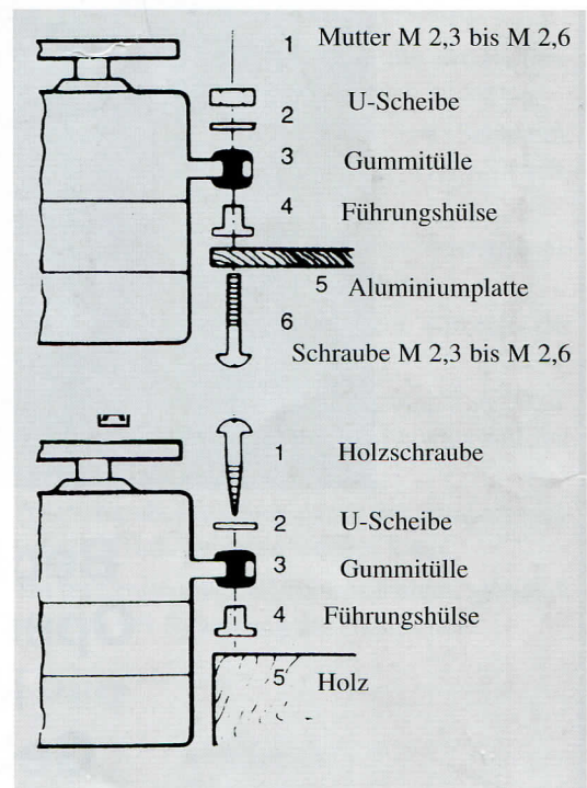
13: Servomontage
